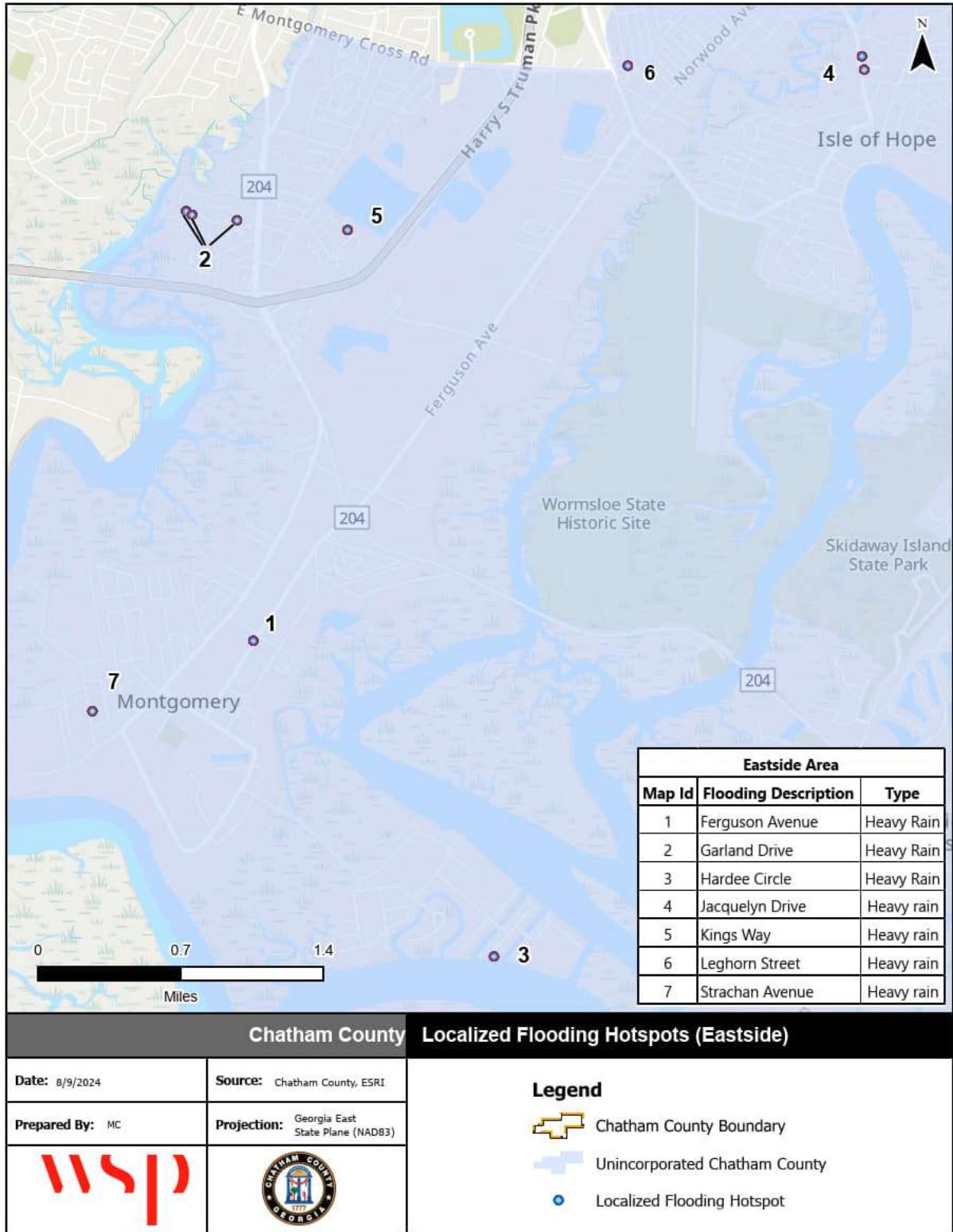
Figure 4-40 - Localized Flooding, Eastside Area
