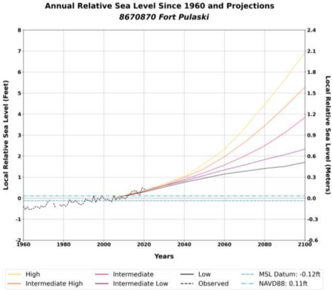
Figure 4-12 - Relative Sea Level Rise Projections for Fort Pulaski, GA
